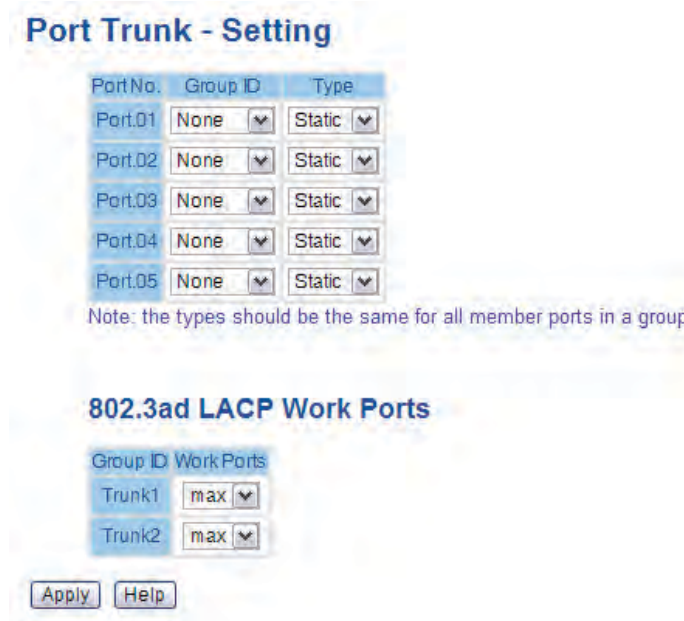
Port Trunk - Setting interface
