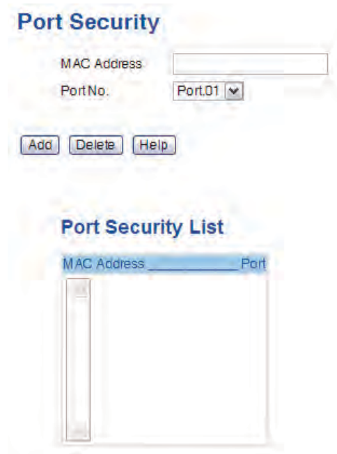
Port Security interface
