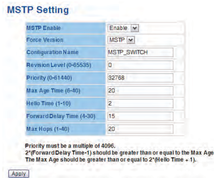
MSTP Setting Interface
