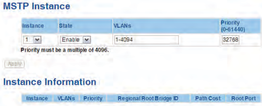
MSTP Instance interface
