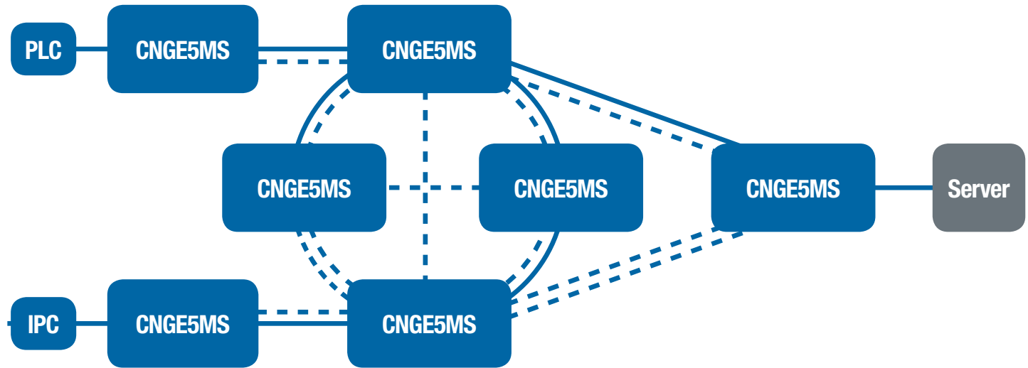
C-RSTP connection
