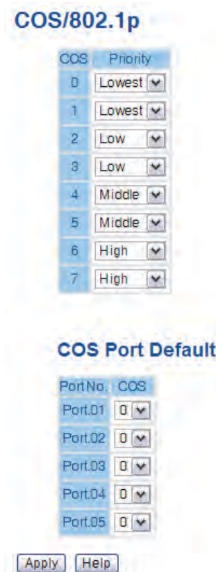
COS/802.1p interface
