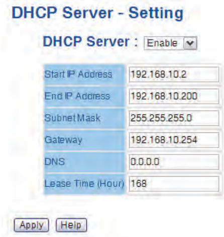
DHCP Server Configuration interface
