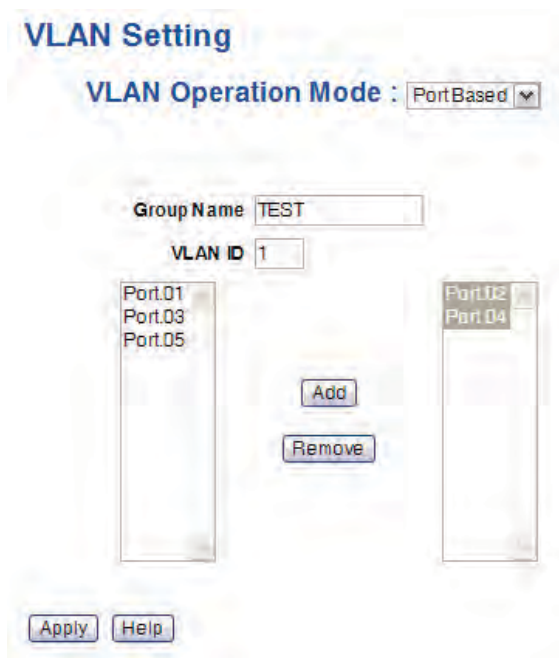
VLAN Configuration - Port Base interface-2
